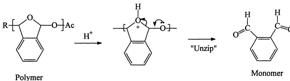
Acid catalyzed scission and unzipping of poly(phthalaldehyde)
